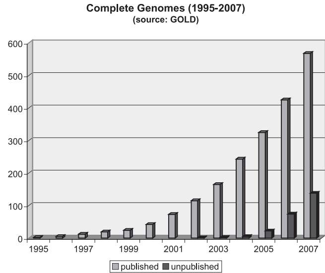
FIG. 1. As sequencing of genomes and metagenomes becomes more commonplace, the practice of publishing a companion "genome paper" in the scientific literature has begun to decline. In 2007, approximately 20% of all completed genomes were without such a publication.
