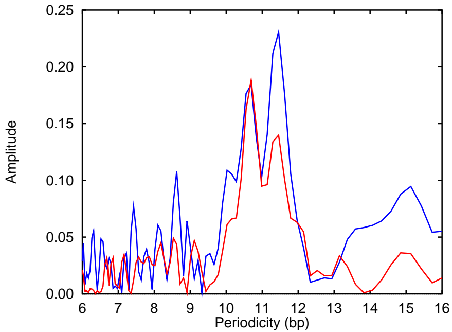
Figure 2b. Periodicity spectrum for the complete genome of thermophilic Archaea P. horikoshii (red) shown together with the Archaea-like sequences from T. maritima (blue).
